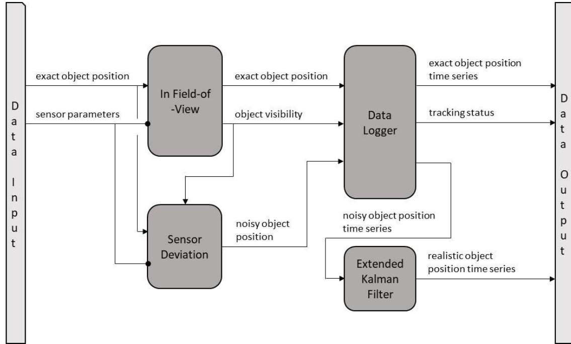
Figure 10: Structure of the sensor model. Parameter-flow (time-independent) is marked with \text{---}\bullet and variable-flow (time-dependent) with \text{---}\rightarrow .
